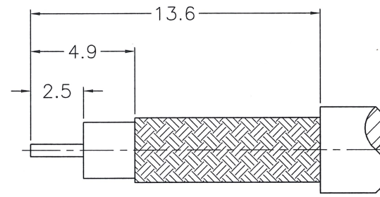
RECOMMENDED CABLE STRIPPING DIM'S (建議剝線尺寸)
